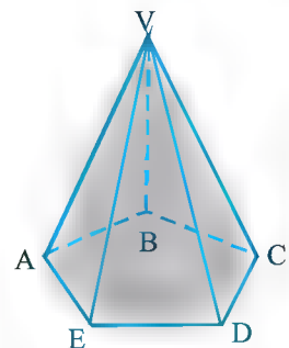
(c) Pentagonal pyramid
